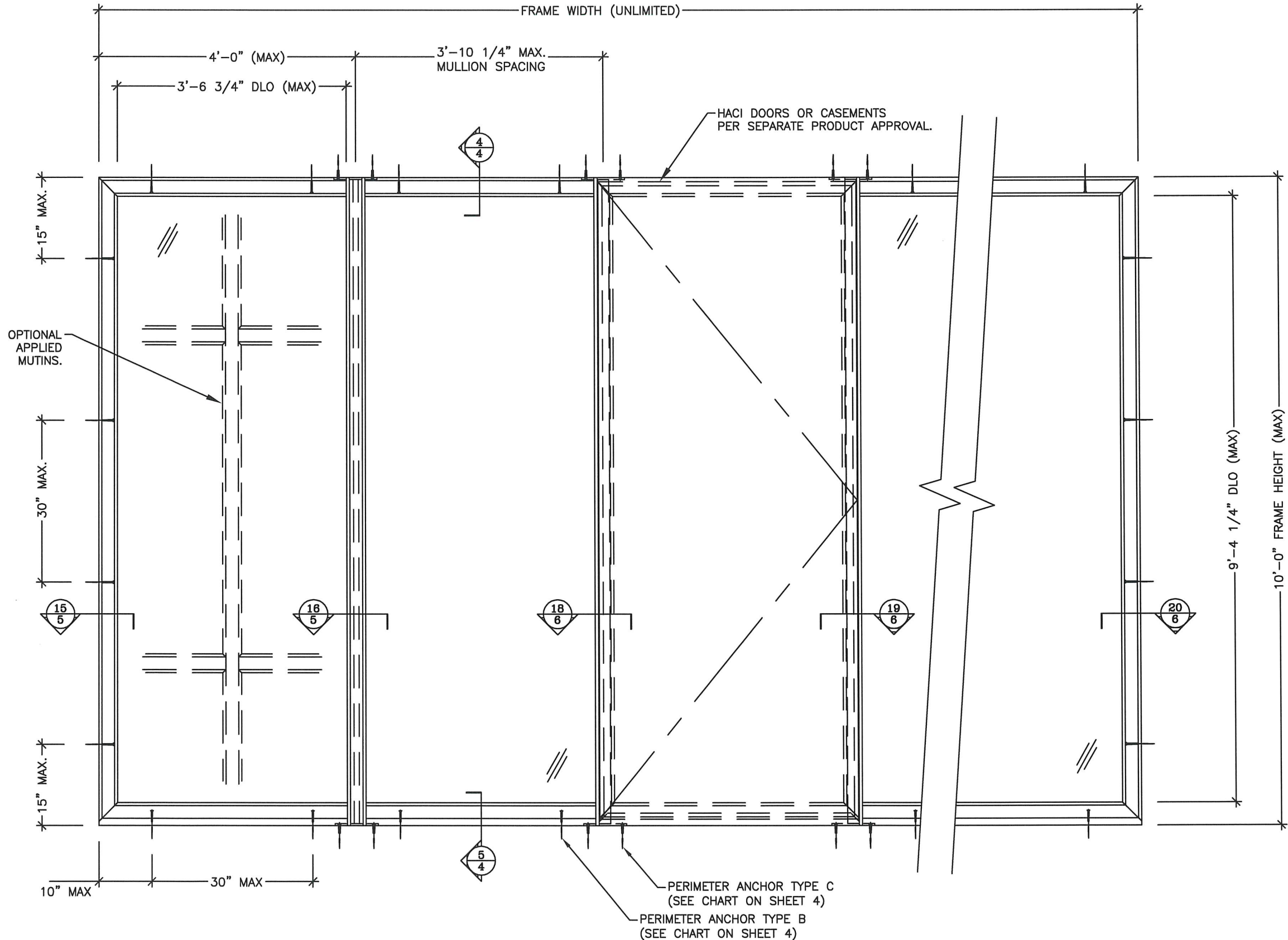
③ WINDOW WALL SYSTEM WITH OUTSWING DOOR (EXTERIOR VIEW)
